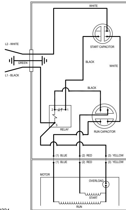
WIRING DIAGRAM FOR MODELS "N803", "N805", "N807", "E803", "E805", "E807" 4/15 thru Current
