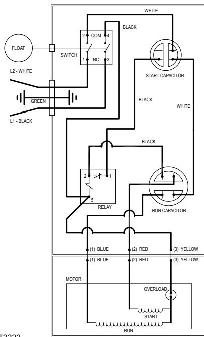
WIRING DIAGRAM FOR MODELS "M803", "M805", "M807", "D803", "D805", "D807" 4/15 thru Current
